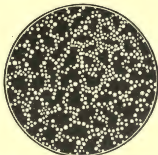
FIG. 15.—Appearance preceding coagulation in a concentrated gold solution. (According to H. Sidenlopf.)
